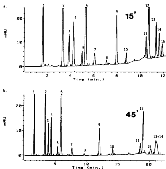
Fig. 1. Experimental chromatograms for the sample studied here. Two runs were initially used for computer simulation (to determine the optimum gradient time or steepness). Conditions: 1–20% B in 15 min (upper trace) and 45 min (lower trace), pH 4.40, respectively. Other conditions as in Section 2.
