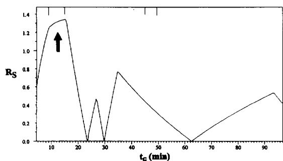
Fig. 2. Resolution map from separations of Fig. 1 (DryLab computer simulation). Arrow indicates preferred gradient time t_G for maximum resolution R_s .
